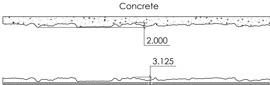
Formliner SECTION A-A
