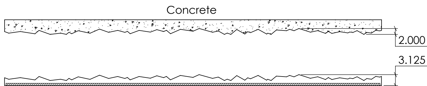
Formliner SECTION A-A
