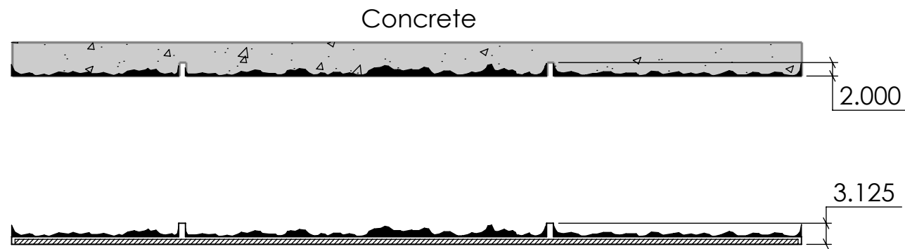
Concrete Formliner SECTION A-A
